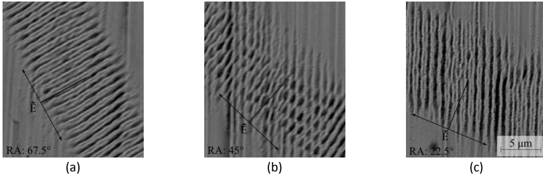
Figure 4: Different regimes during the LSFL generation on linear polished surfaces. The double arrow indicates the polarization direction of the incident laser (a) for RA = 67.5° LSFL follow the normal of the polarisation, (b) for RA = 45° irregular LSFL formation and (c) for RA = 22.5° LSFL follow the polishing direction. All structures are generated on stainless steel with a surface roughness of Ra = 126 nm with a fluence of 0.5 J/cm 2 .
