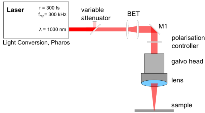
Figure 1: Experimental setup for surface treatment: M1 is a mirror, BET is a beam expander telescope, and polarization control is obtained by a half wave plate
