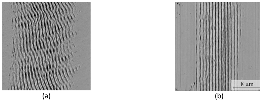
Figure 3: Periodic surface structures on a) undefined b) linear (vertical) polished surface
