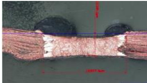
Fig. 10b. 20 layers of 8 \mu\text{m} Copper foil, 260 Watts @ 0.24 m/min
