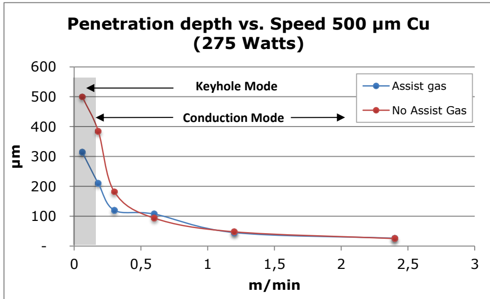
Fig. 8. Bead-on-plate results for 500 \mu\text{m} Copper @ 275 Watts (with and without assist gas)
