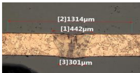
Fig. 7a. Cross section results for 254 \mu\text{m} Copper @ 275 Watts, 0.3 m/min – keyhole mode Regime
