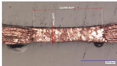
Fig. 10a. 10 layers of 8 \mu\text{m} Copper foil, 130 Watts @ 0.72 m/min
