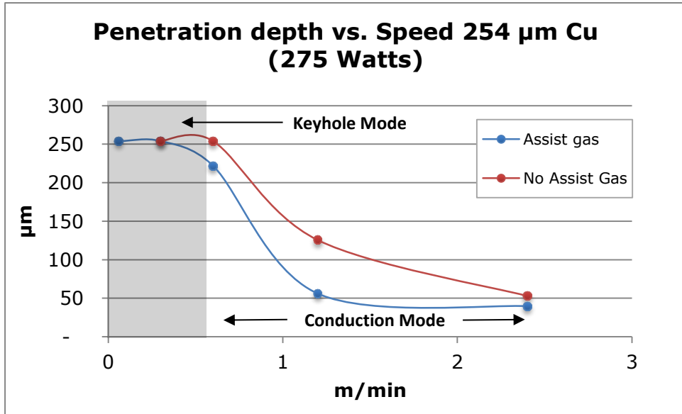
Fig. 6. Bead-on-plate results for 254 \mu\text{m} Copper @ 275 Watts (with and without assist gas)
