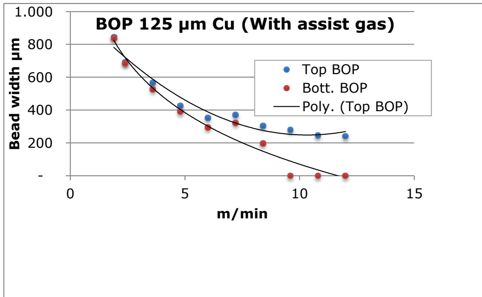
Fig. 4. Bead-on-plate results for 125 μm Copper @ 275 Watts
