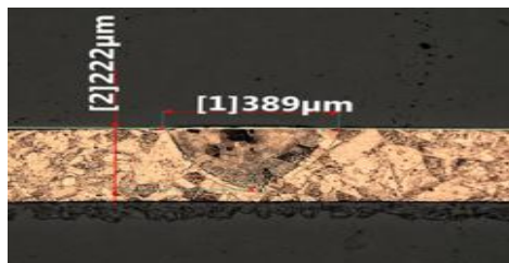
Fig. 7b. Cross section results for 254 \mu\text{m} Copper @ 275 Watts, 0.6 m/min – conduction mode
