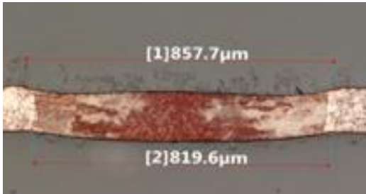
Fig. 5a. Cross section results for 125 μm Copper @ 275 Watts, 1.92 m/min
