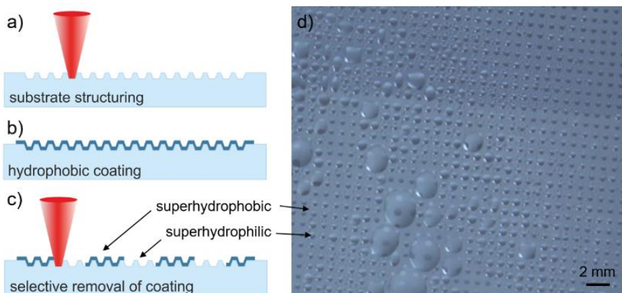
Fig. 1. a) to c) Fabrications steps of the patent-pending ClearSurface™ process. d) Droplets collected from a nebulizer on the Superhydrophobic/Superhydrophilic micropattern.
