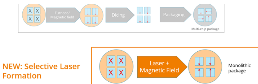
Fig. 3. Magnetic sensor production by multi-chip-packaging.
