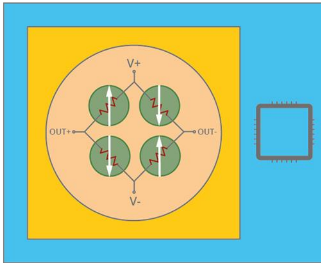
Fig. 1. Four magnetic sensors (green circles) with two different orientations in a Wheatstone bridge (amber circle) as part of a monolithic integrated sensor chip (blue).
